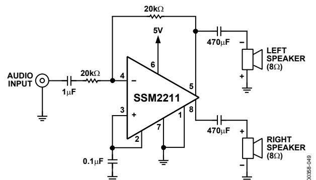
Figure 49. SSM2211 Used as a Dual-Speaker Amplifier
