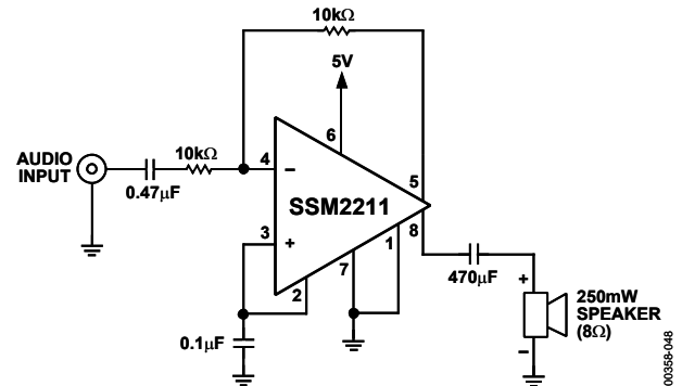
Figure 48. Single-Ended Output Application
